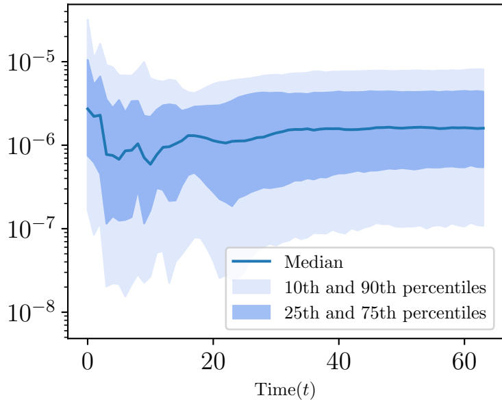
Euler residuals squared ( \varepsilon^2 ) with \phi(\text{Moments})
