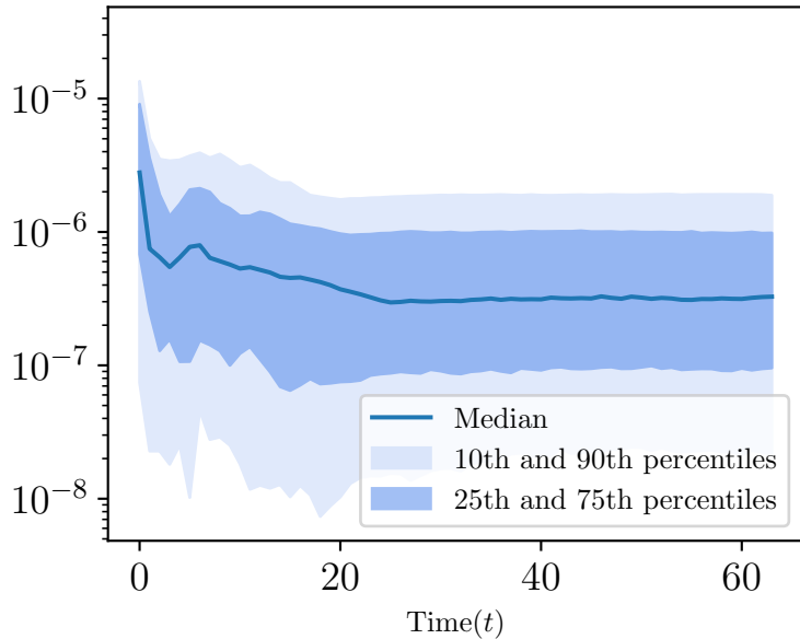
Euler residuals squared ( \varepsilon^2 ) with \phi(\text{ReLU})
