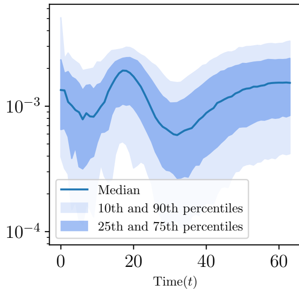
Policy errors ( \epsilon_{\text{rel}} ) with \phi(\text{Moments})
