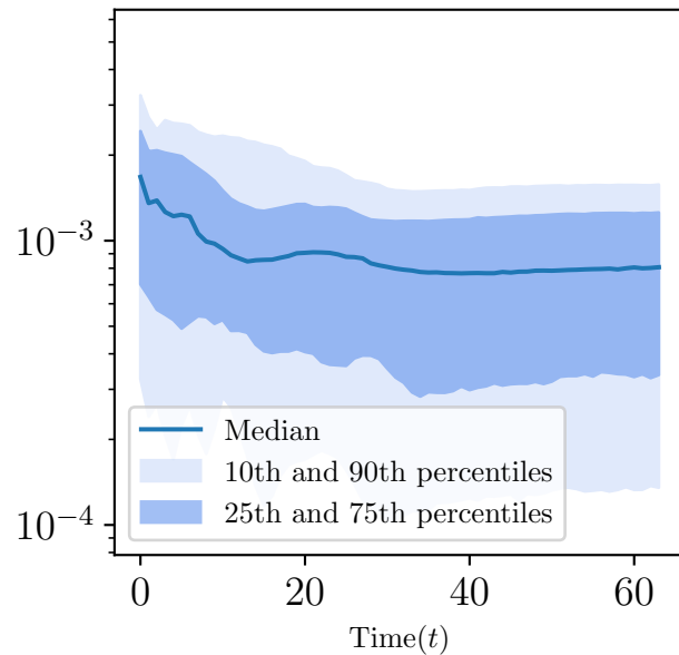
Policy errors ( \epsilon_{\text{rel}} ) with \phi(\text{ReLU})
