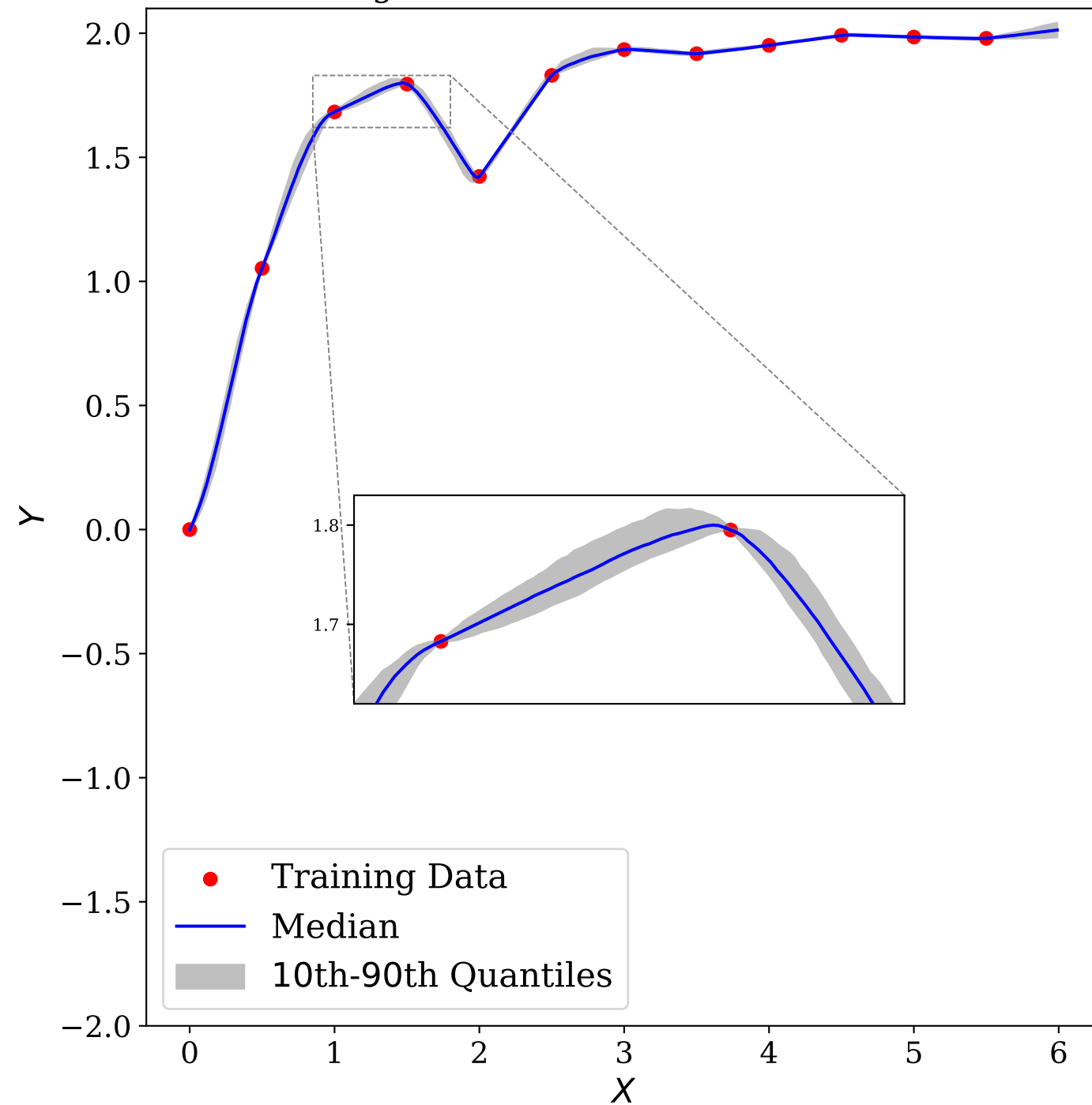
After training: Initialization with Uniform Distribution
