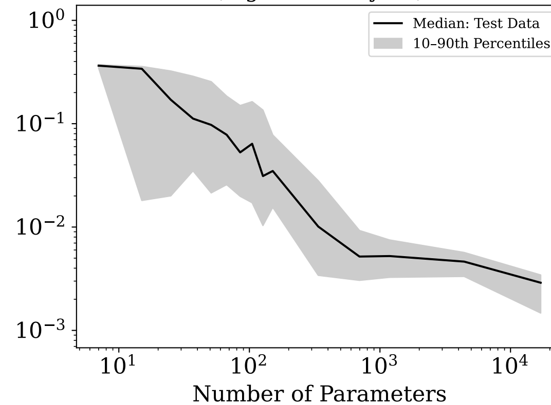
Median Abs Relative Error (Sigmoid, 2 layers)
