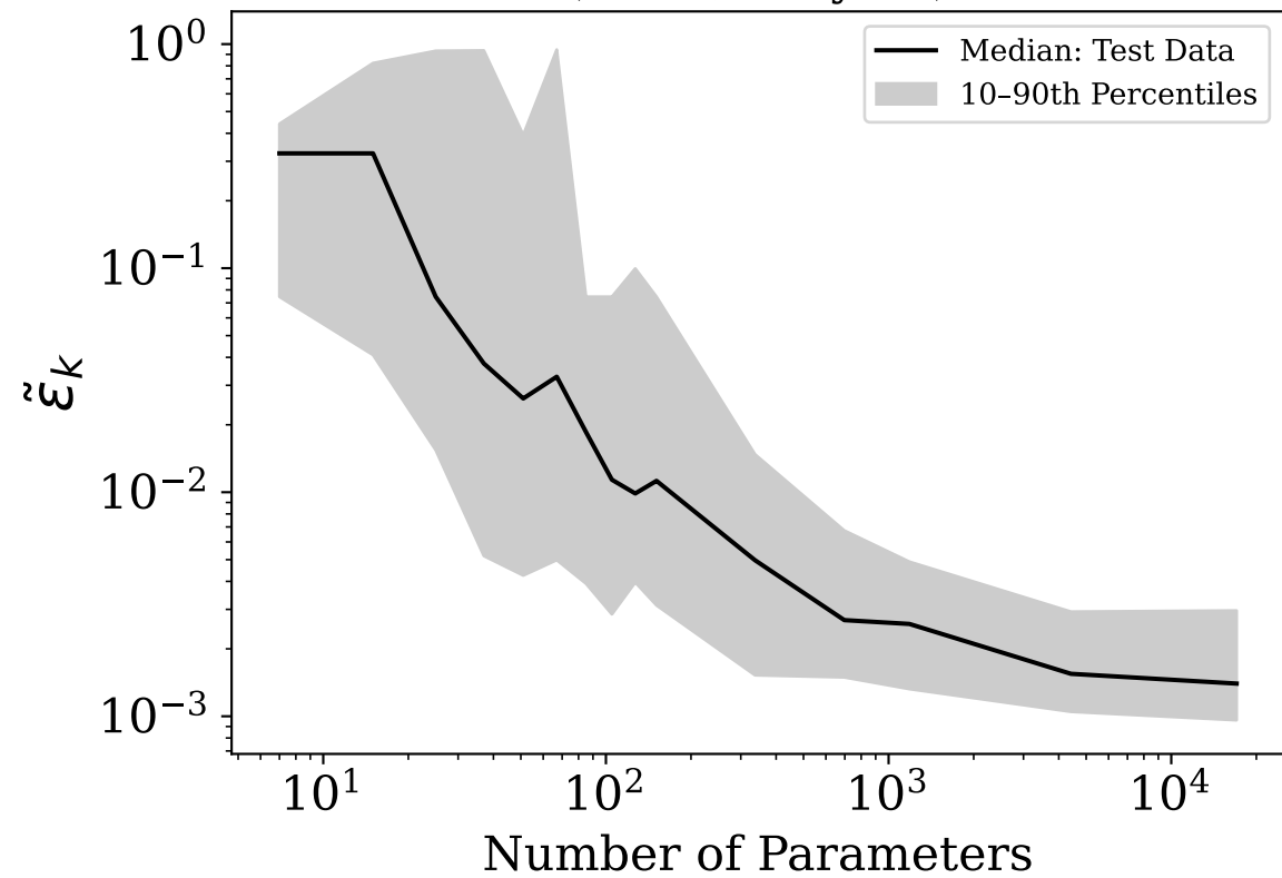
Median Abs Relative Error (ReLU, 2 layers)
