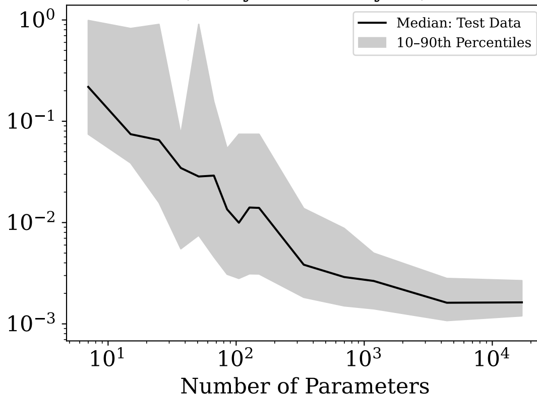
Median Abs Relative Error (Leaky ReLU, 2 layers)
