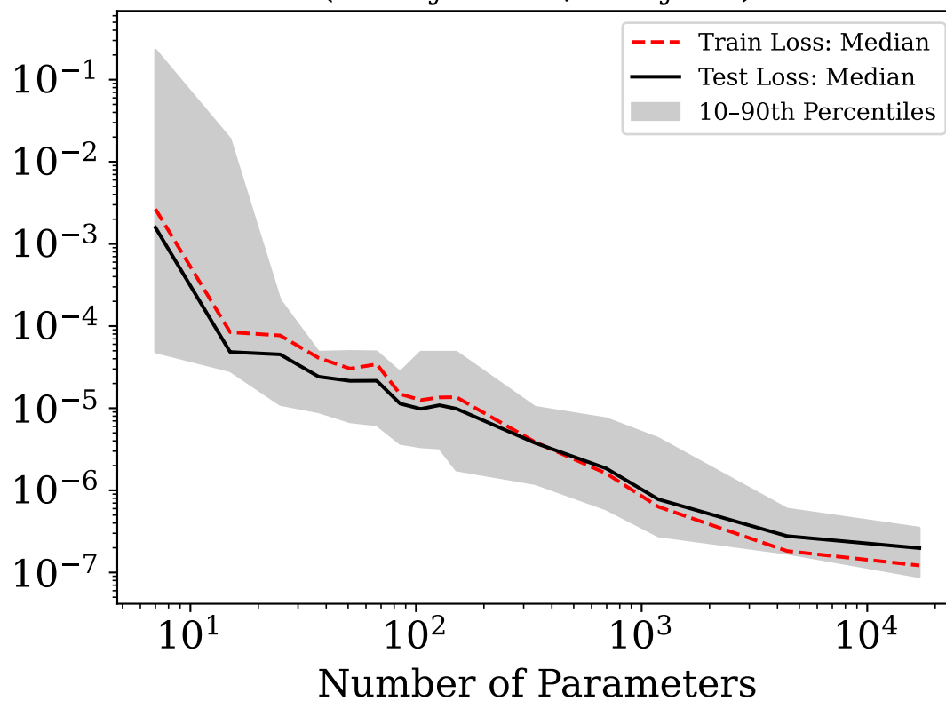
RBC Model: Train vs Test Loss (Leaky ReLU, 2 layers)
