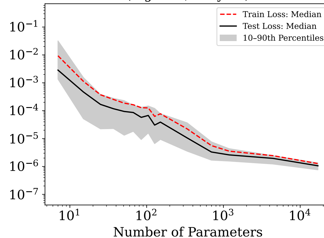
RBC Model: Train vs Test Loss (Sigmoid, 2 layers)
