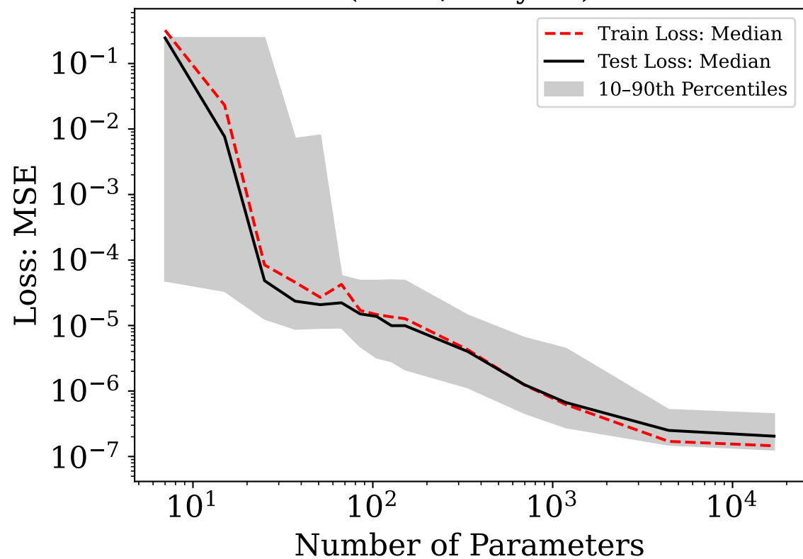
RBC Model: Train vs Test Loss (ReLU, 2 layers)
