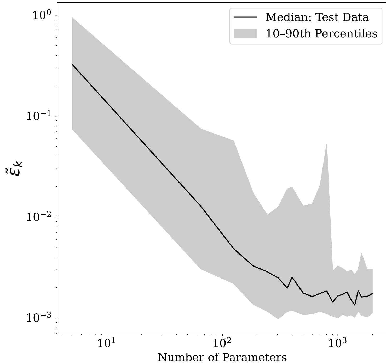
RBC Model: Median Abs Relative Error
