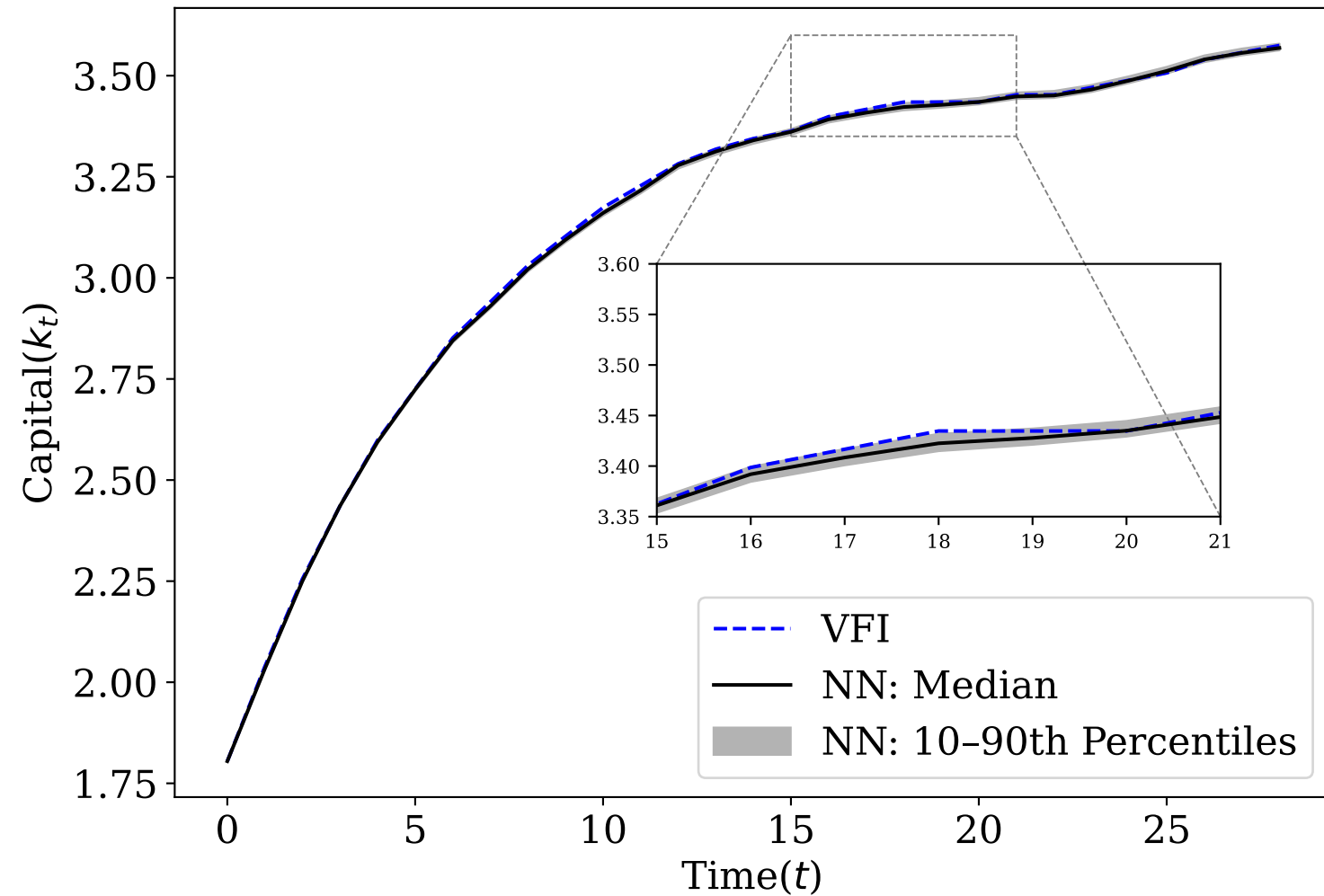
RBC Model: Capital Path, VFI vs NN ( H = 512 )
