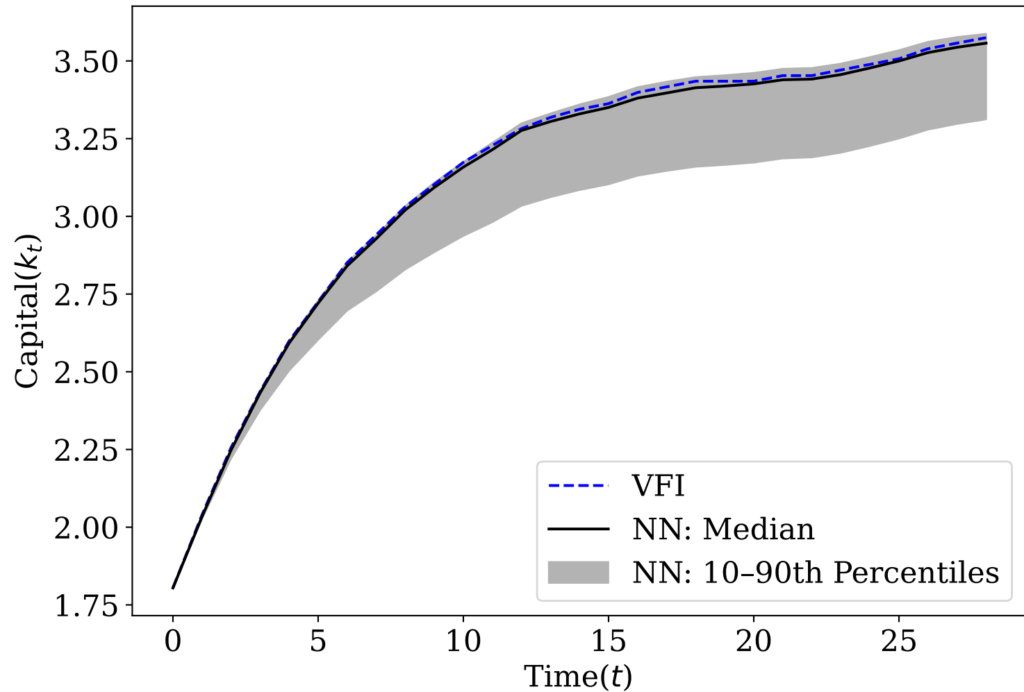
RBC Model: Capital Path, VFI vs NN ( H = 32 )
