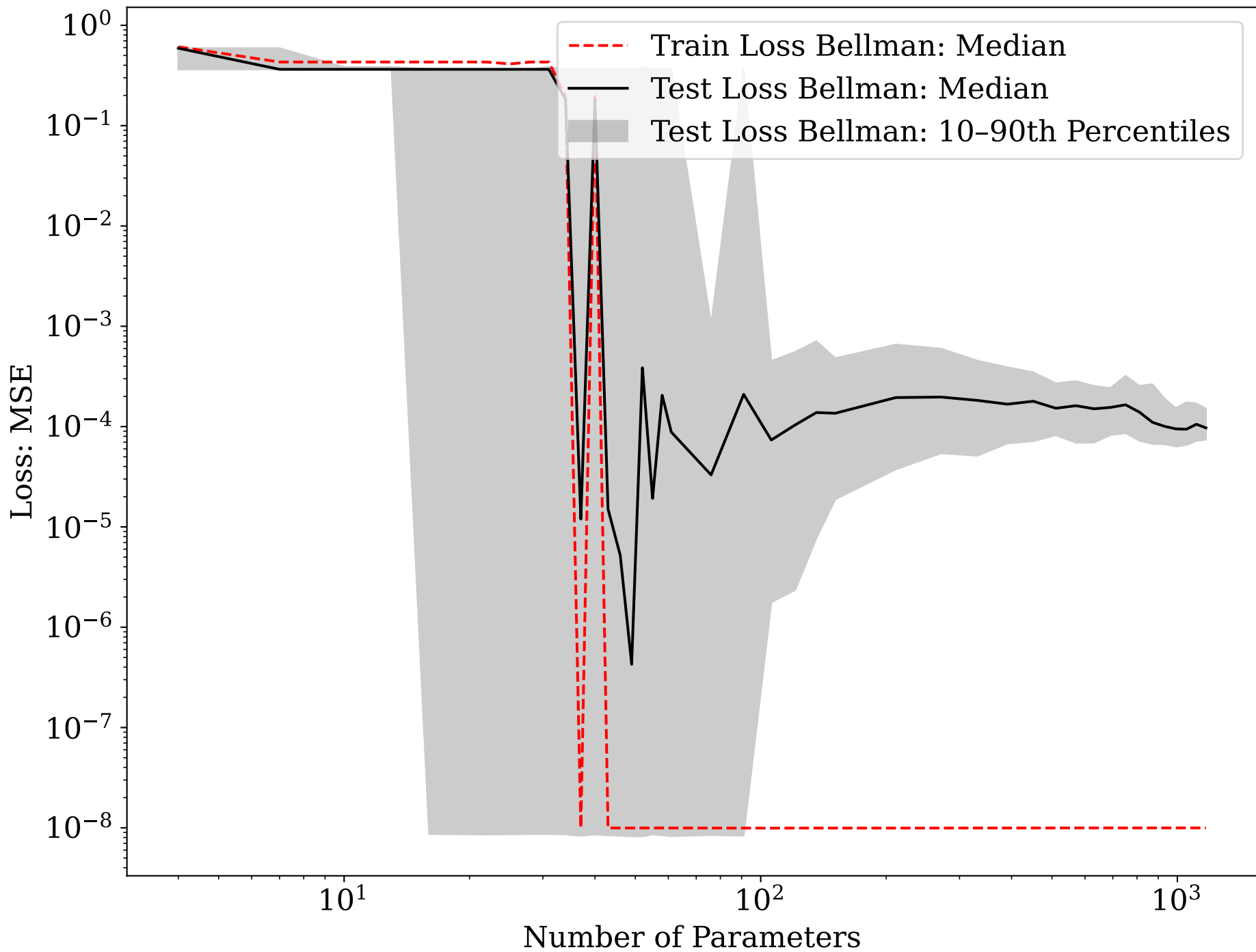
McCall Model: Train vs Test Loss
