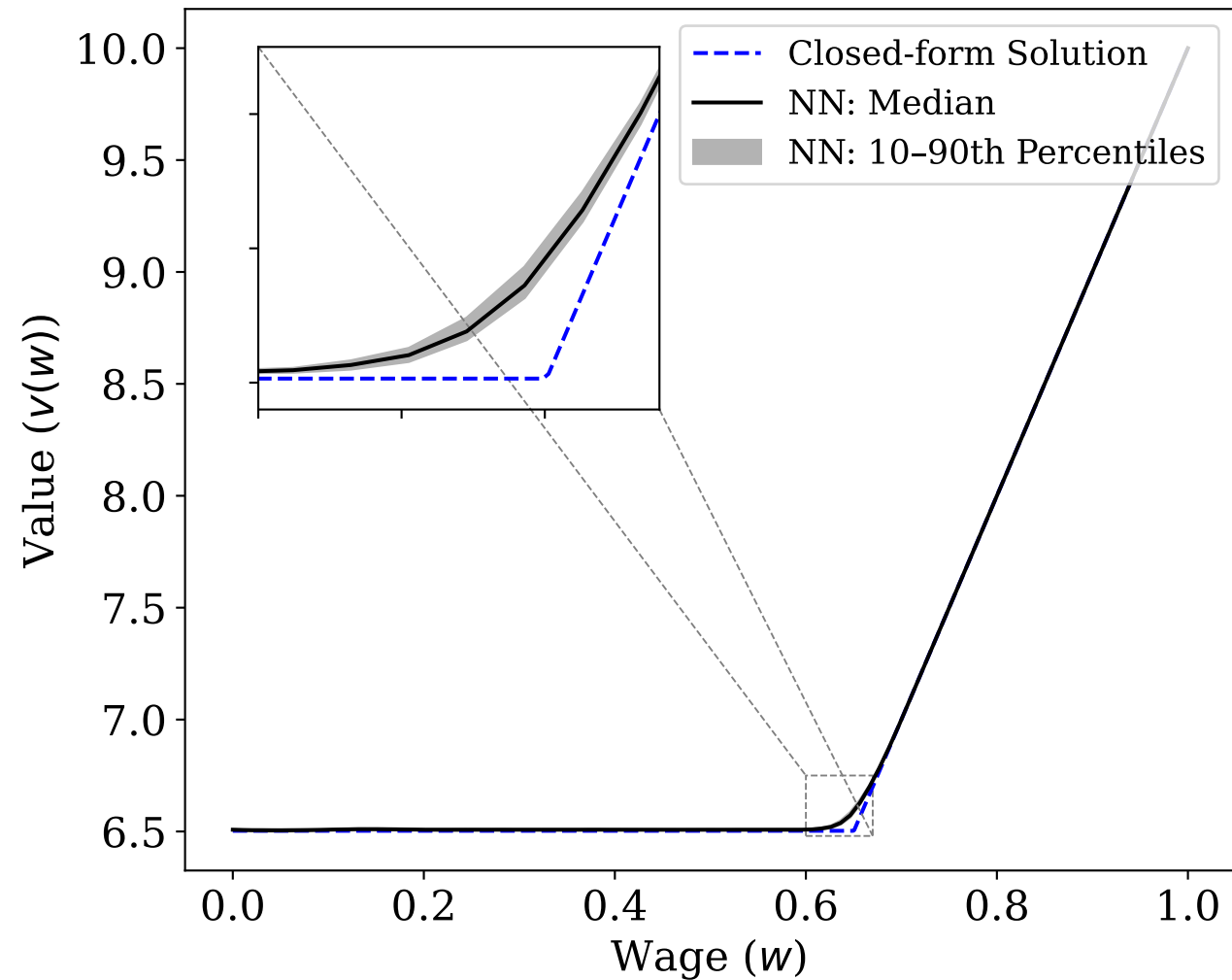
McCall Model: Closed-form vs NN ( H = 512 )
