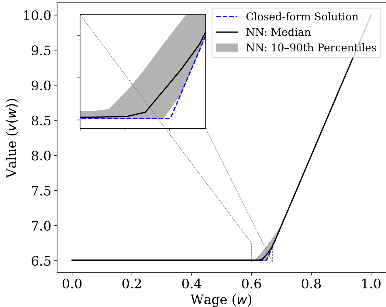
McCall Model: Closed-form vs NN ( H = 24 )
