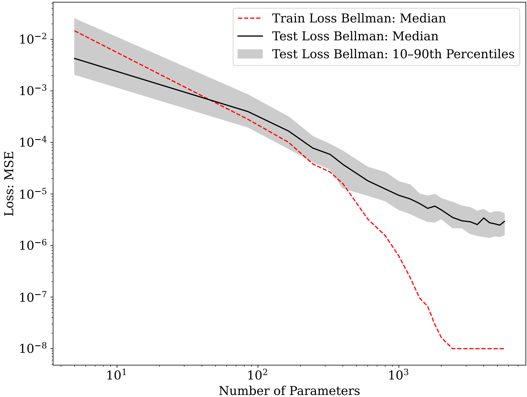
LQ Model: Train vs Test Loss (Bellman Residuals)
