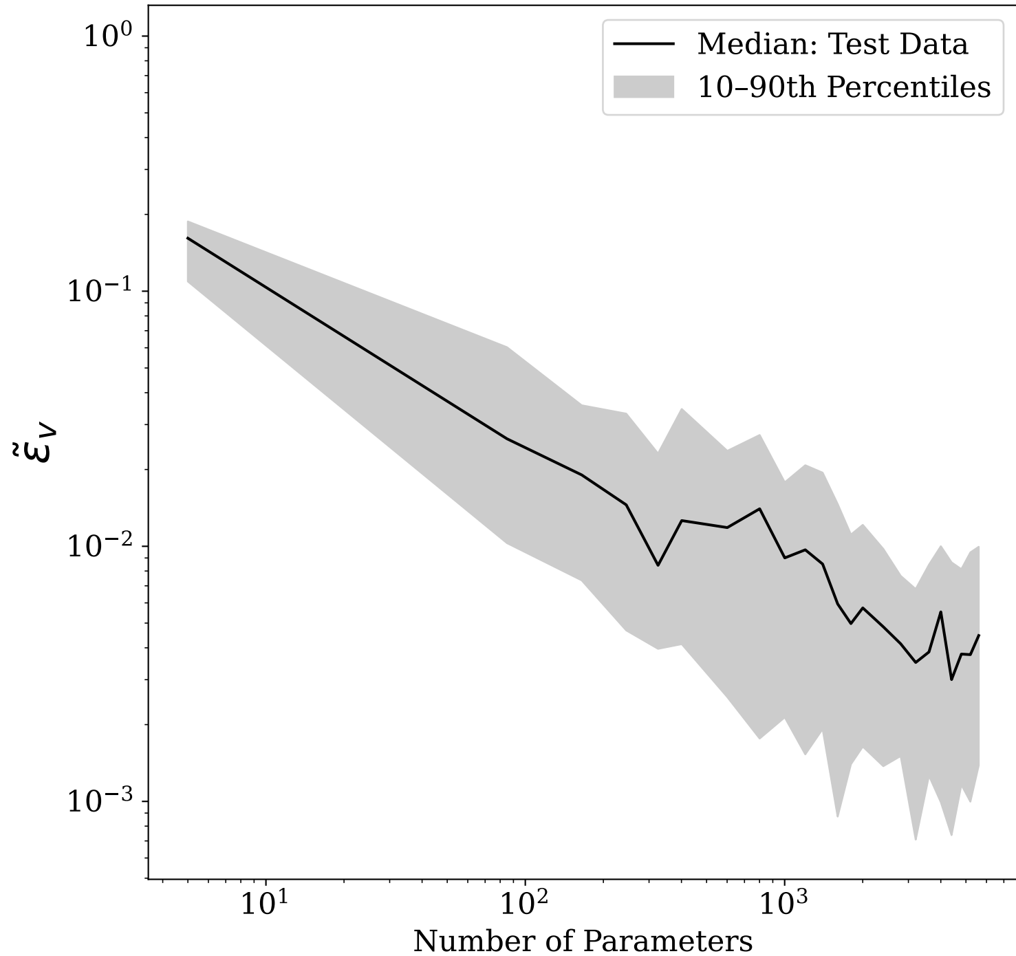
LQ Model: Value Function, Median Abs Relative Error
