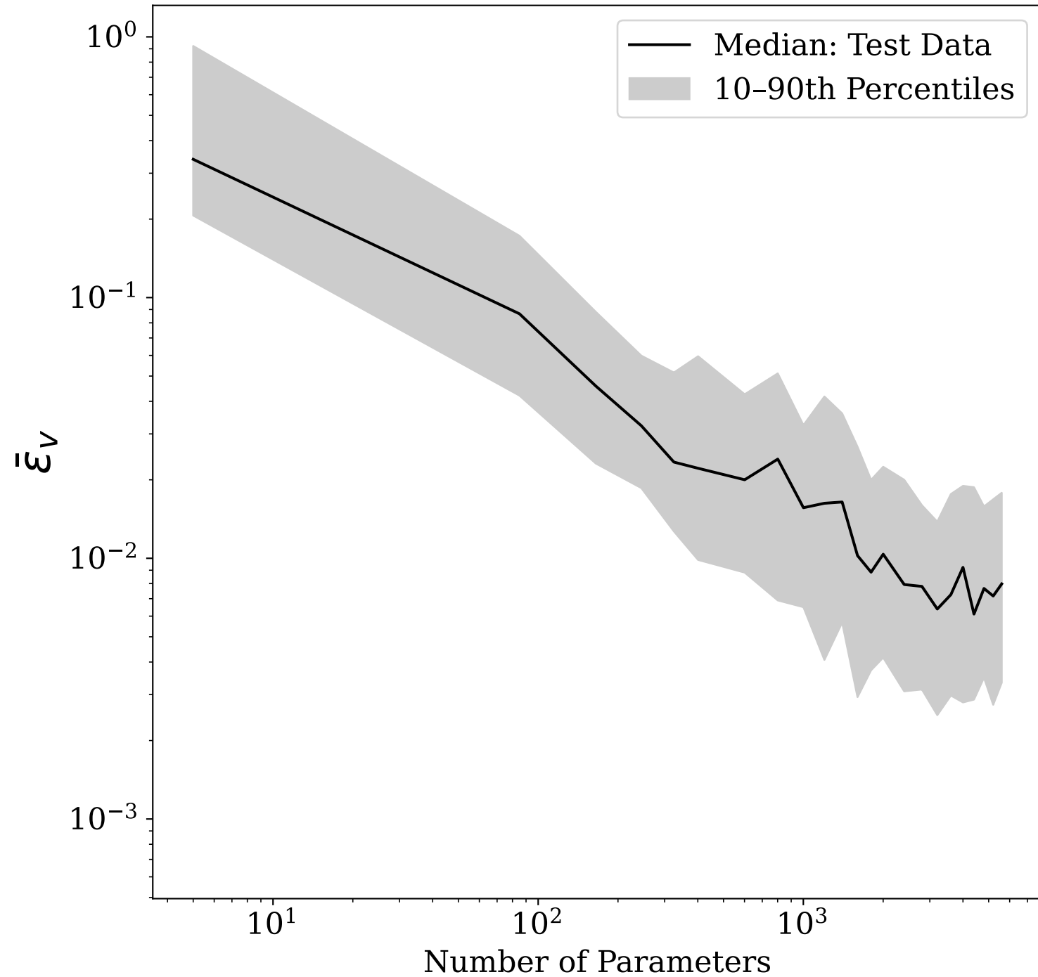
LQ Model: Value Function, Max Abs Relative Error
