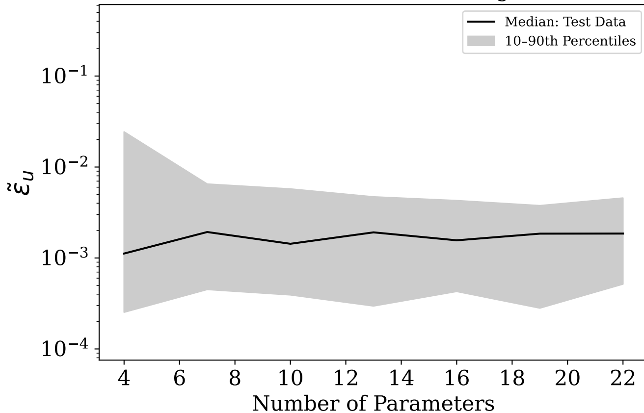
Median Abs Relative Error (Sigmoid)
