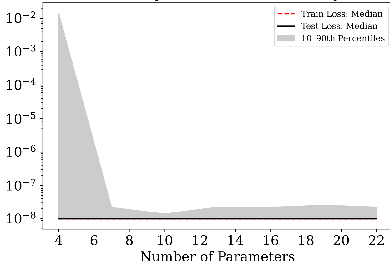
LQ Model: Policy, Train vs Test Loss (Leaky ReLU)
