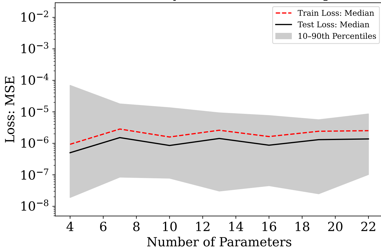
LQ Model: Policy, Train vs Test Loss (Sigmoid)
