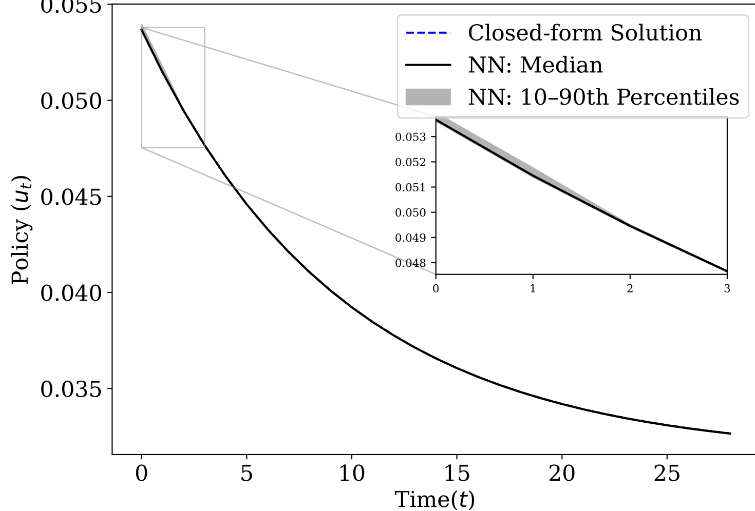
LQ Model: Policy Path, Closed-form vs NN ( H = 32 )
